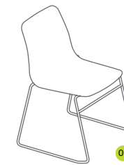
POLLY-CH-SL Polly chair on sled base metric (mm) W524 D530 H785 seat 450 imperial (in) W20.5 D21 H31 seat 17.5
